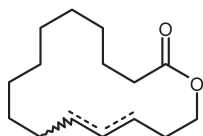
Oxacyclohexadec-12-en-2-one, (12E)-
